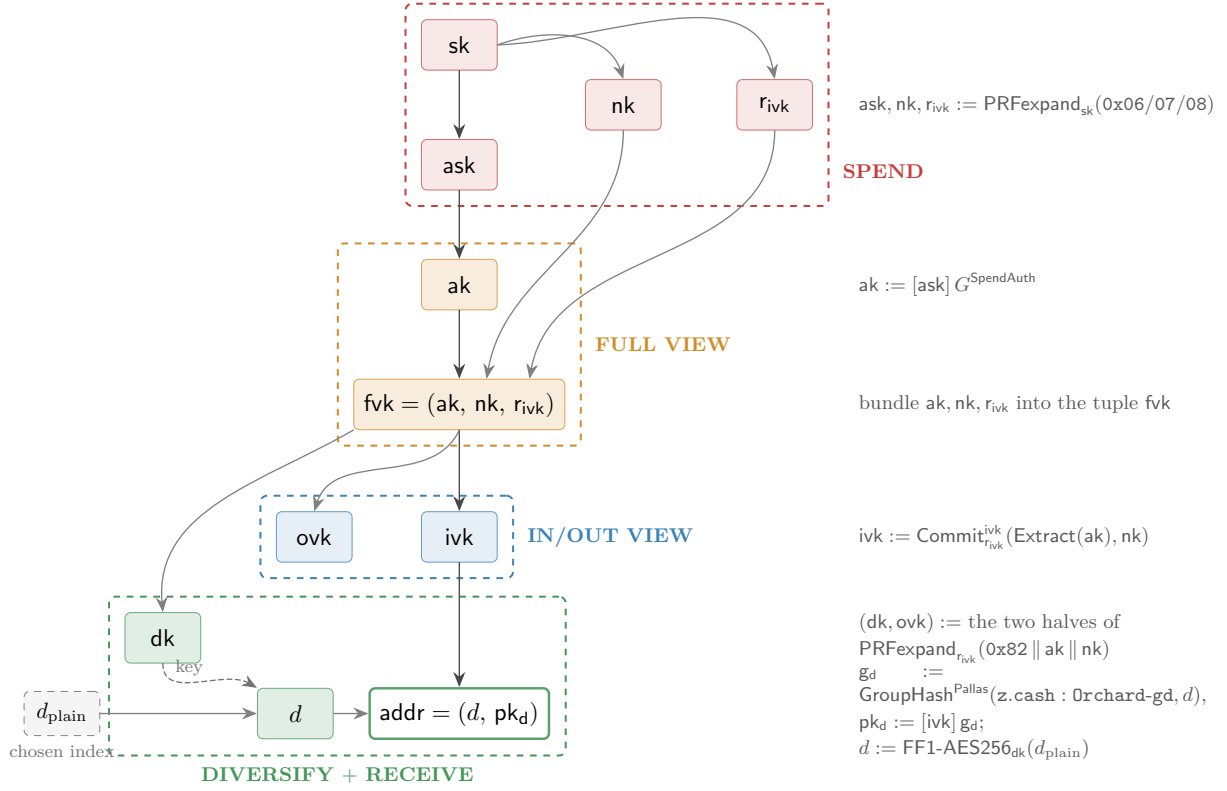
Figure 1: The Orchard key hierarchy as a capability ladder, read top to bottom. Each arrow is a one-way derivation; the right-hand gutter shows the operation that produces the child from its parent(s). The dk and ovk keys are the two halves of one \text{PRFexpand}_{fvk} output (tag 0x82 , input ak \parallel nk ); they play different roles and land in different tiers — ovk is the outgoing viewing key, grouped with the incoming viewing key ivk as the IN/OUT viewing tier, whereas dk is the diversifier key, which sits in the address layer because it generates diversified addresses. Concretely d is the format-preserving encryption \text{FF1-AES256} of a chosen index d_{\text{plain}} under the key dk (the dashed edge marks dk entering as the cipher key), and pk_d = [ivk] g_d , so the address binds both keys. Every node is secret key material except the chosen index d_{\text{plain}} , the diversifier d , and the diversified address (unshaded) — the address (d, pk_d) , and with it d , is the only value the protocol ever publishes (shading marks tier membership, not secrecy) — in particular the viewing keys fvk , ivk , ovk are secret : “viewing” names what they let the holder do, not that the protocol publishes them. Each dashed tier holds a strictly weaker capability than the one above, so a holder may receive a lower-tier key without gaining the powers above it. Drawn to match Definition 2.4.
