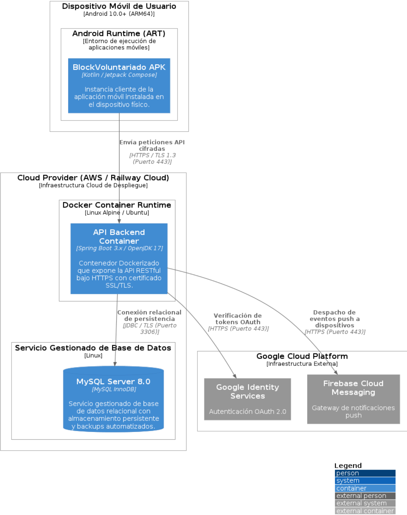
Diagrama de Despliegue (C4 Deployment) - BlockVoluntariado
