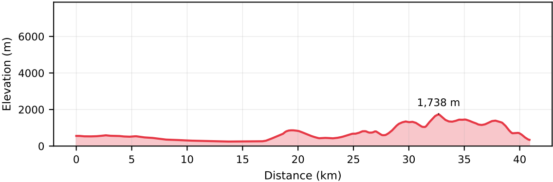
Profile A - A' · 84.71°E, South → North
