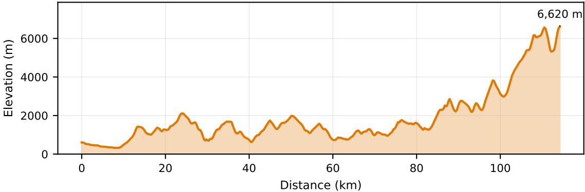
Profile B - B' · 85.78°E, South → North
