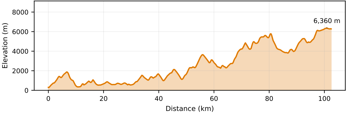
Profile B - B' · 84.50°E, South → North
