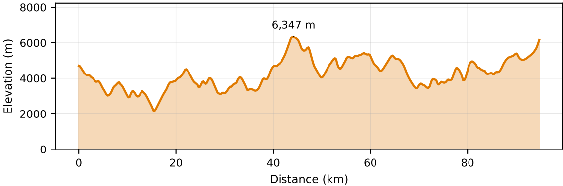
Profile B - B' · 82.87°E, South → North
