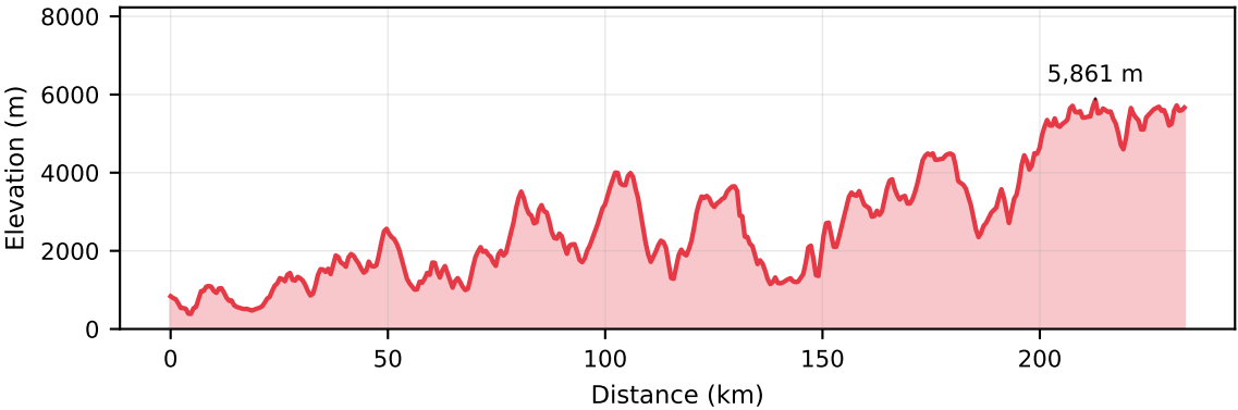
Profile A - A' · 81.79°E, South → North
