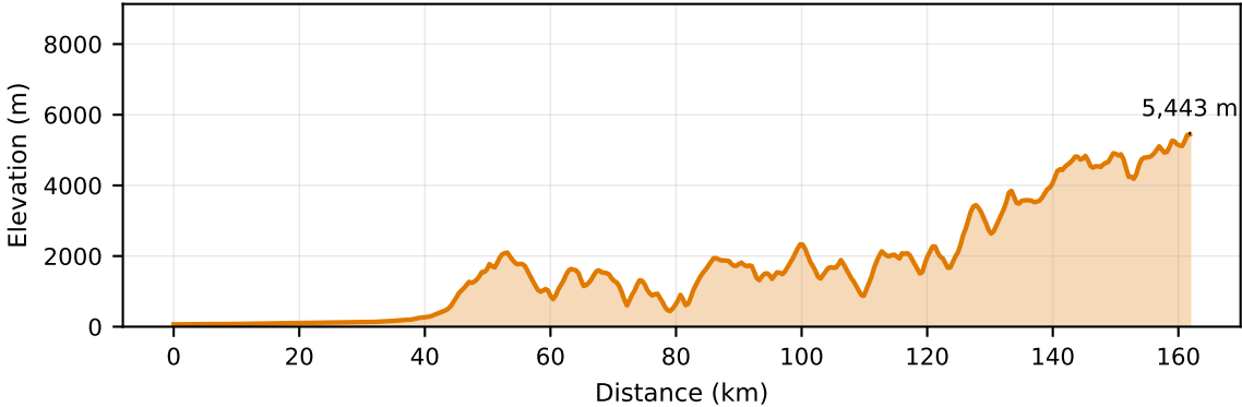
Profile B - B' · 87.59°E, South → North
