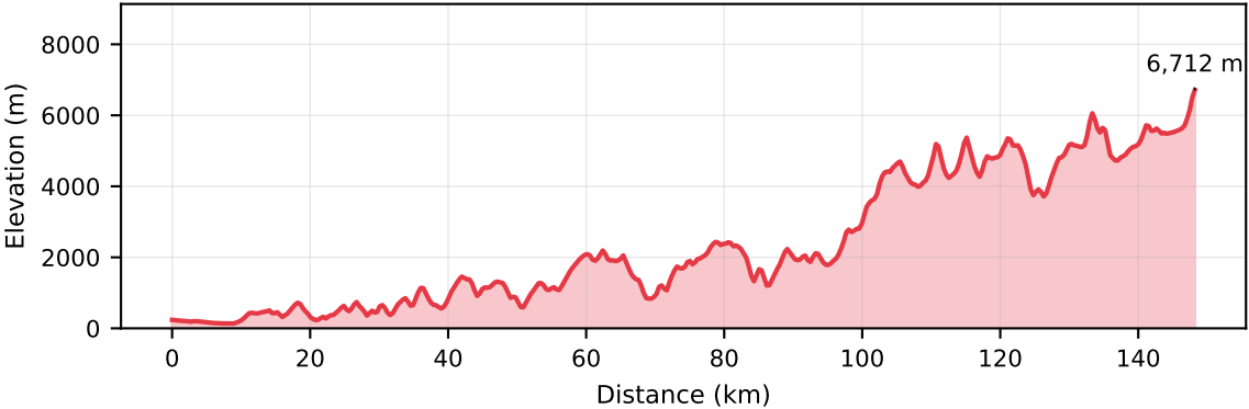
Profile A - A' · 86.77°E, South → North
