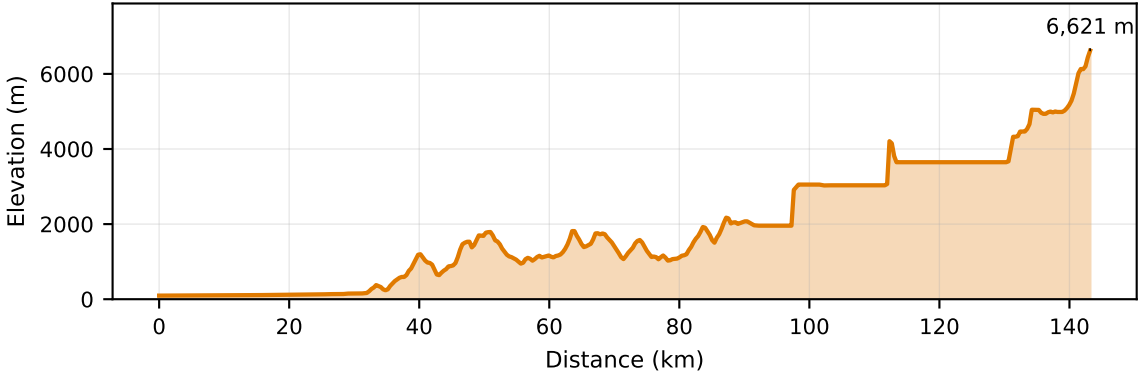
Profile B - B' · 83.14°E, South → North
