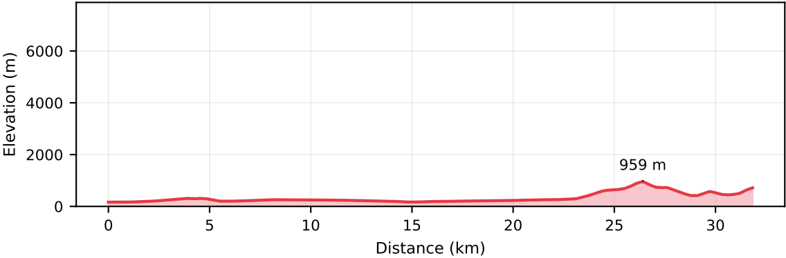
Profile A - A' · 81.95°E, South → North
