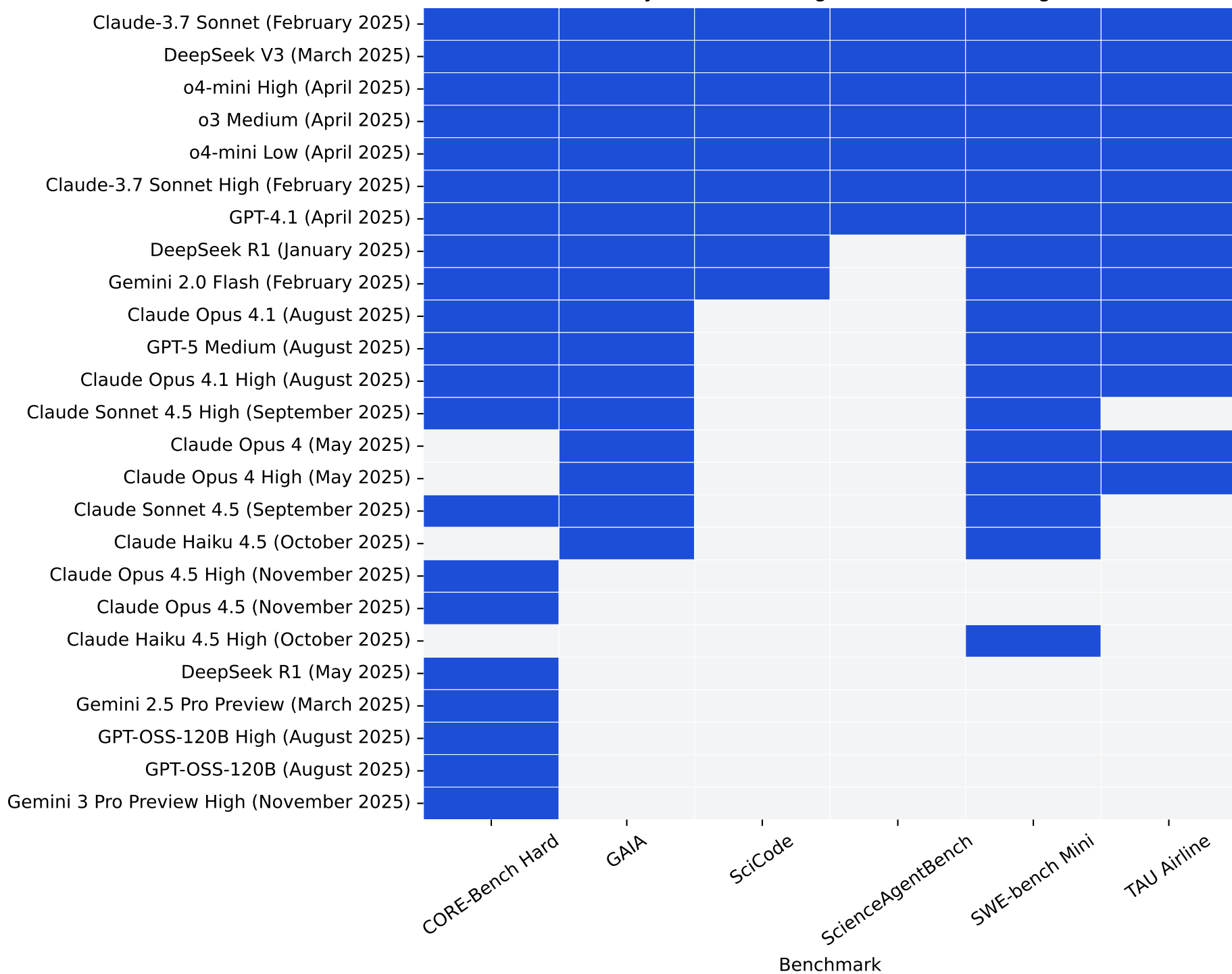
Primary-cohort coverage: HAL Generalist Agent
