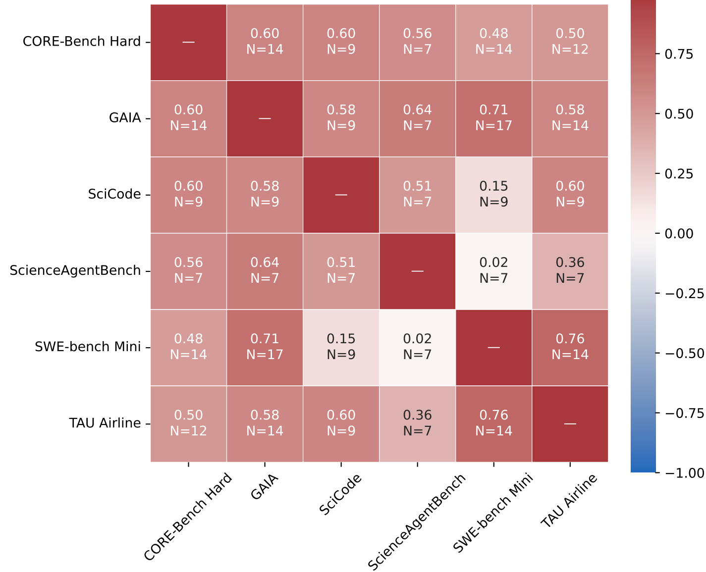
Accuracy-rank transfer (Spearman \rho )
