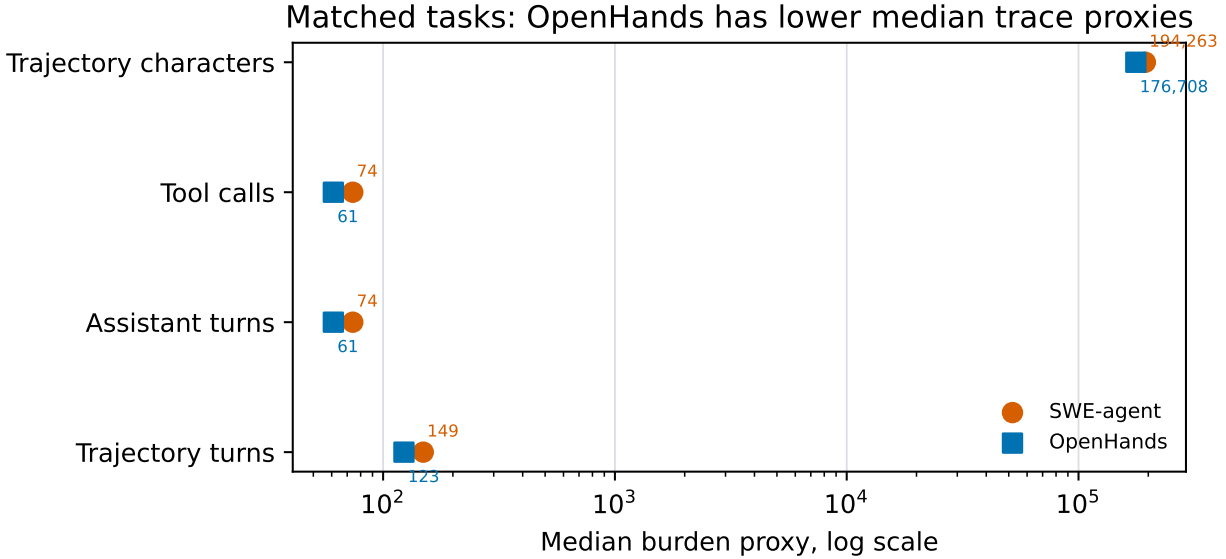
Figure 4: Matched MiniMax-M2.5 task pairs in the Open-SWE boundary sample ( N = 977 ). Markers show scaffold medians on a log scale for trace proxies, not tokens or dollars.
