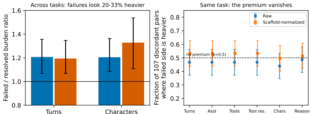
Figure 3: The failure-cost premium is a composition artifact. Left: across tasks, failed trajectories appear 20–33% heavier (bootstrap intervals). Right: on the 107 matched pairs where scaffolds disagree on the identical task, the failed side is heavier about half the time, raw or scaffold-normalized, consistent with no premium.
