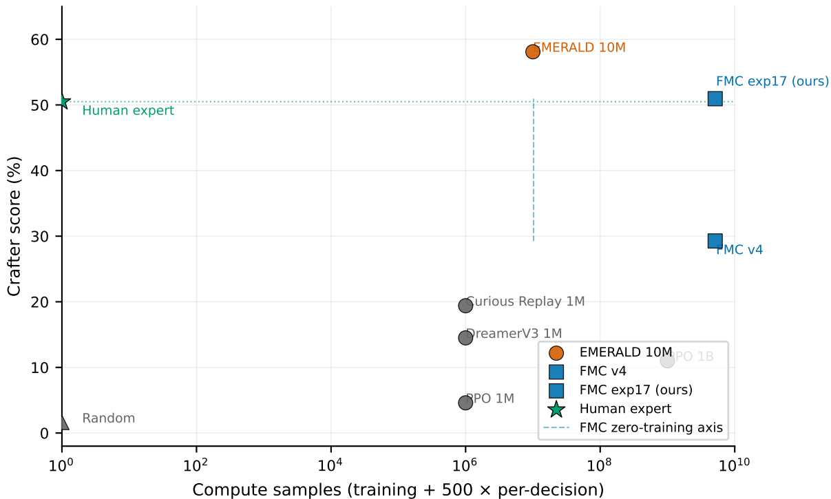
Sample-efficiency Pareto: zero-training FMC reaches human-expert
