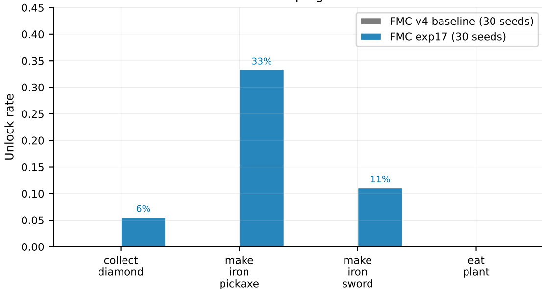
v4-blocker unlock rates: shaping unblocks 3 of 4 blockers
