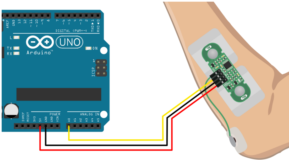
Fig. 5: Connections with Arduino UNO R3
