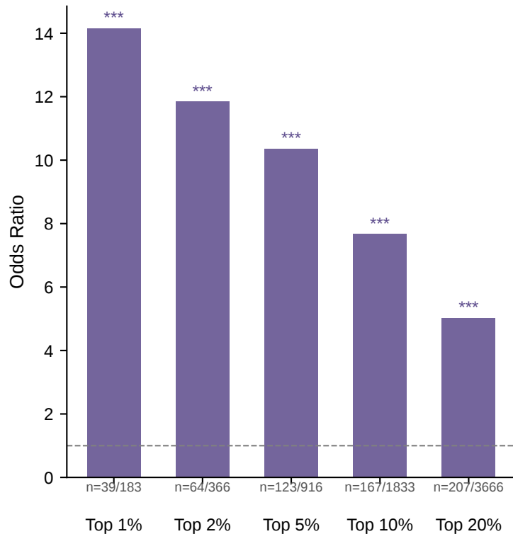
Odds Ratio by Top-k% Cutoff
