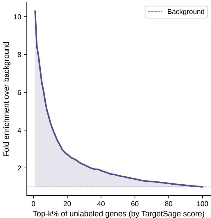
ChEMBL Phase 2/3 Target Enrichment
