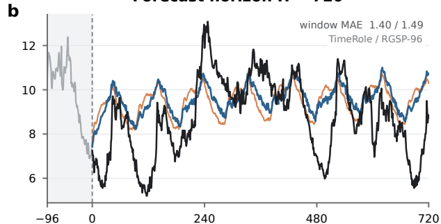
Forecast horizon H = 720
