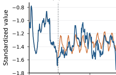
(a) TimeRole
