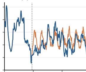
(c) iTransformer
