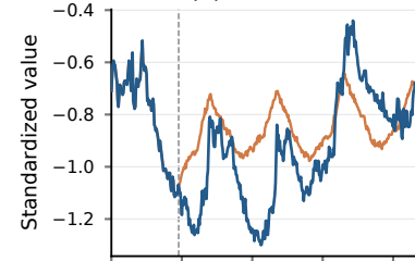
(a) TimeRole
