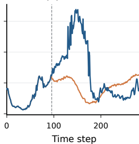
(h) DLinear
