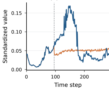
(e) MSGNet
