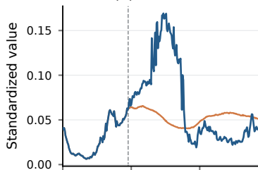
(a) TimeRole
