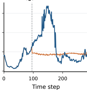
(g) TimesNet
