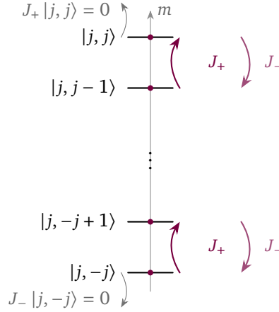
Figure 1.1: The weight ladder of the spin- j representation. The J_z -eigenvalues m = j, j - 1, \dots, -j label the rungs; the raising and lowering operators J_{\pm} = J_x \pm iJ_y step between adjacent rungs, J_{\pm} |j, m\rangle = \sqrt{j(j+1) - m(m \pm 1)} |j, m \pm 1\rangle . The string is finite because J_+ annihilates the highest weight |j, j\rangle and J_- the lowest |j, -j\rangle ; matching the two terminations forces 2j \in \mathbb{Z}_{\geq 0} and fixes the dimension at 2j + 1 . Half-integer j (e.g. j = \frac{1}{2}, \frac{3}{2} ) are exactly the representations of \mathfrak{su}(2) that fail to descend to SO(3) .
