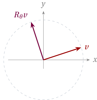
Figure 2: A rotation moves every nonzero vector off its own line, so over \mathbb{R} it has no eigenvector. Over \mathbb{C} its eigenvalues are e^{\pm i\theta} .
