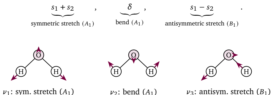
Figure 1.1: The three normal modes of water with their Mulliken labels. Small arrows on the oxygen keep the centre of mass fixed. The two A_1 coordinates mix; the patterns shown are the symmetry-adapted coordinates whose 2 \times 2 reduced matrix determines the two A_1 frequencies.
