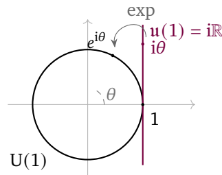
Figure 1.1: The exponential map of the circle group: \exp wraps the tangent line u(1) = i\mathbb{R} around \text{U}(1) with period 2\pi — bijective near the identity, not injective globally, surjective onto the connected compact group.
