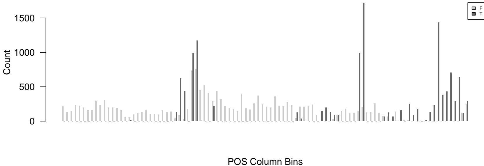
Barplot Comparing TANGLED Frequencies Across Bins
