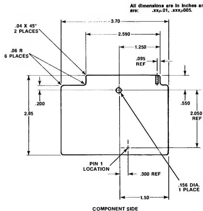
Figure 4-5A. 13/26 Pin Connector
