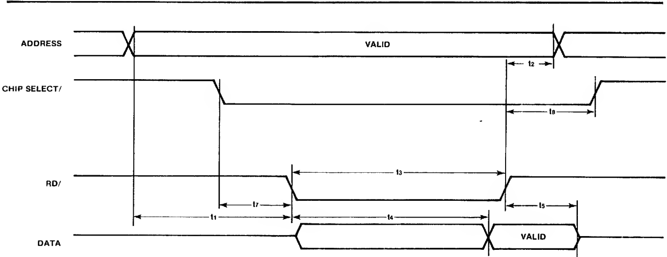
Figure 5-2. READ Timing
