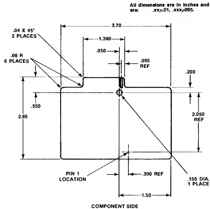
Figure 4-5A. 13/26 Pin Connector
