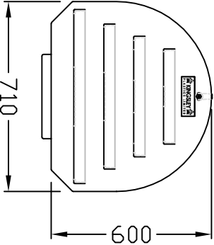
ACCESS PANEL
