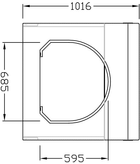
COVER
