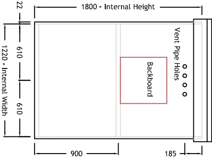
LH & RH SIDE ELEVATION - SCALE 40:1 (A3)
