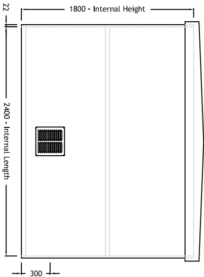
REAR ELEVATION - SCALE 40:1 (A3)
