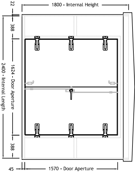
FRONT ELEVATION - SCALE 40:1 (A3)
