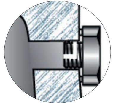
BR - Plugged Boss for Block & Bleed Tapped BSP.P
