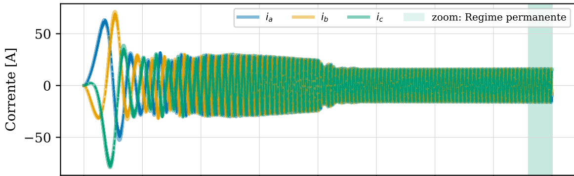
L3 — Full-stack — V/f 2 s: correntes (— Top_HIL, - - C indep.)
