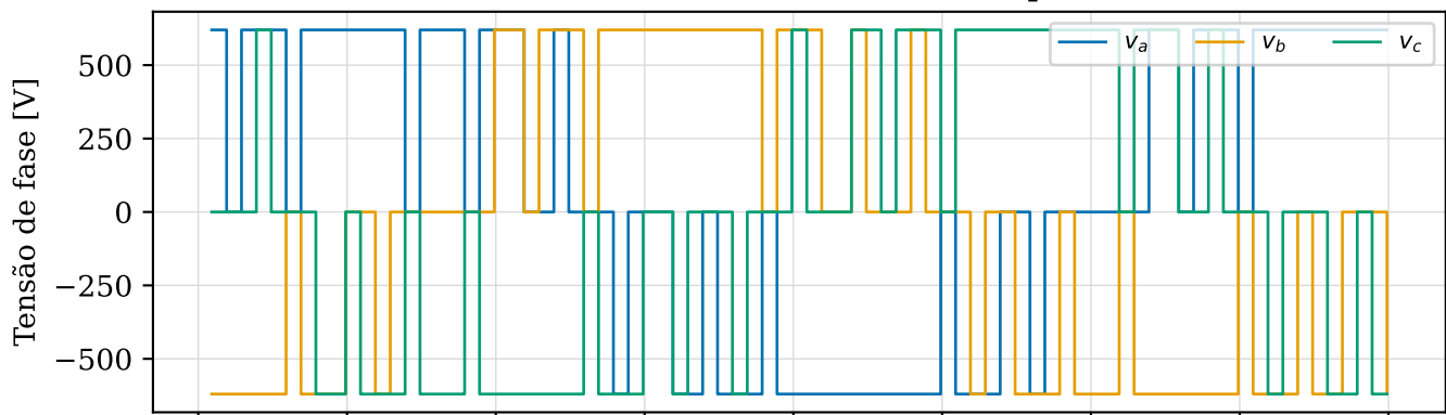
L3 — Full-stack — V/f 2 s: estímulo PWM → resposta, 1900–1920 ms
