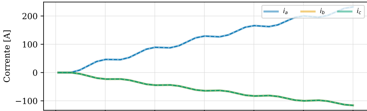
L3 — PWM replay — Seno 6 ms: correntes (— Top_HIL, - - C (replay))
