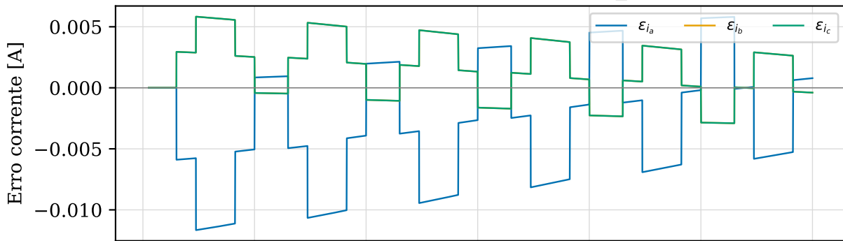
L3 — PWM replay — Seno 6 ms: erro Top_HIL — C (replay)
