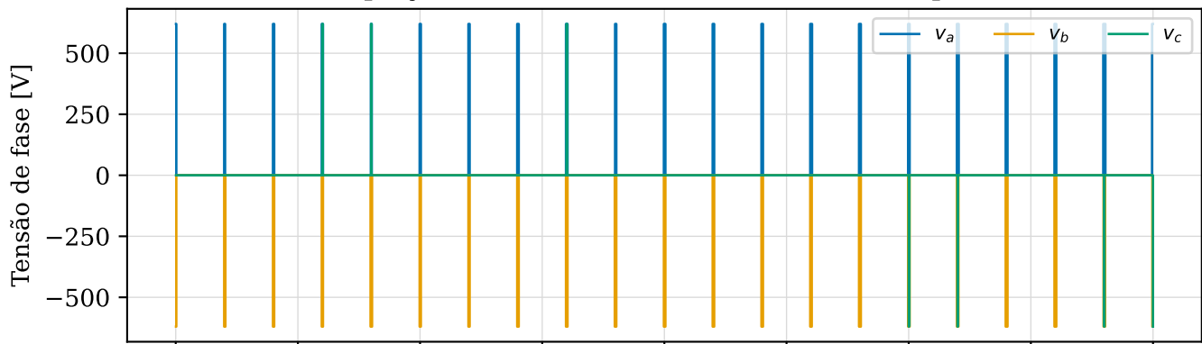
L3 — PWM replay — V/f 50 ms: estímulo PWM → resposta, 25-45 ms
