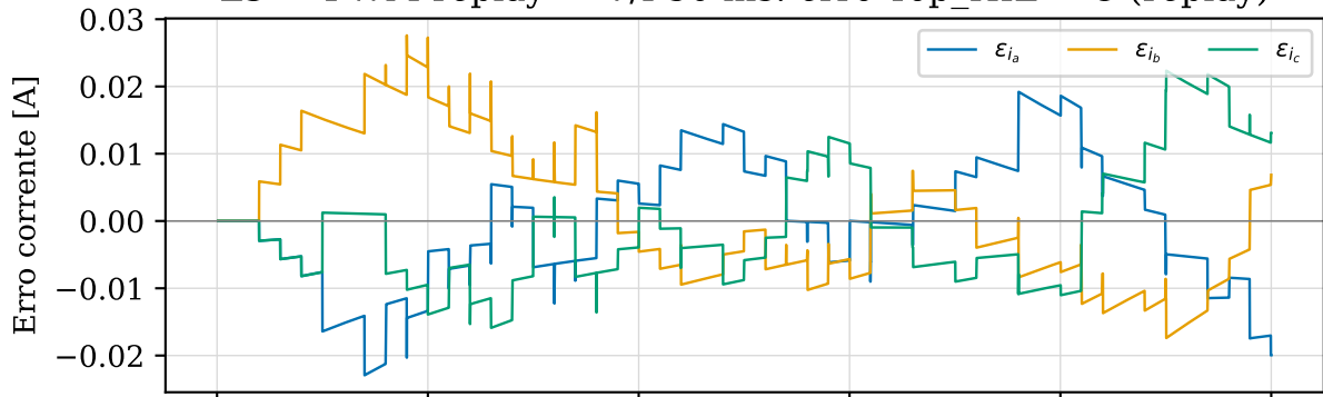
L3 — PWM replay — V/f 50 ms: erro Top_HIL – C (replay)
