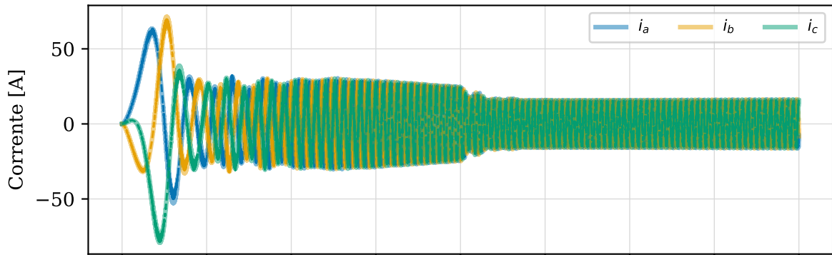
L3 — PWM replay — V/f 2 s: correntes (— Top_HIL, - - C (replay))
