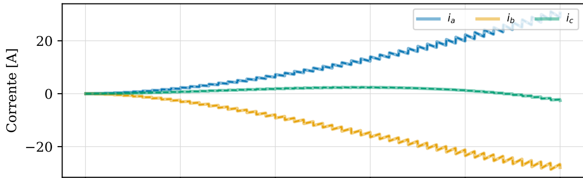
L3 — PWM replay — V/f 50 ms: correntes (— Top_HIL, - - C (replay))
