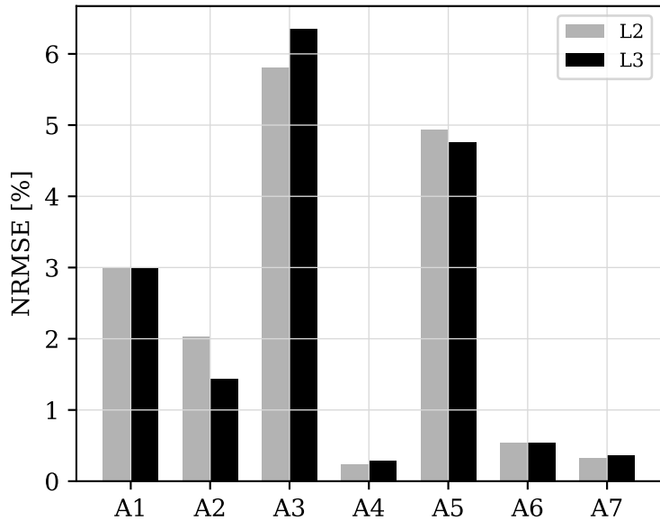
i_\alpha NRMSE
