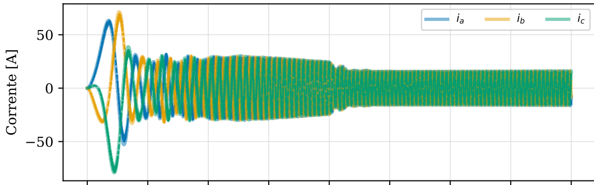
L3 — Full-stack — V/f 2 s: correntes (— Top_HIL, - - C indep.)
