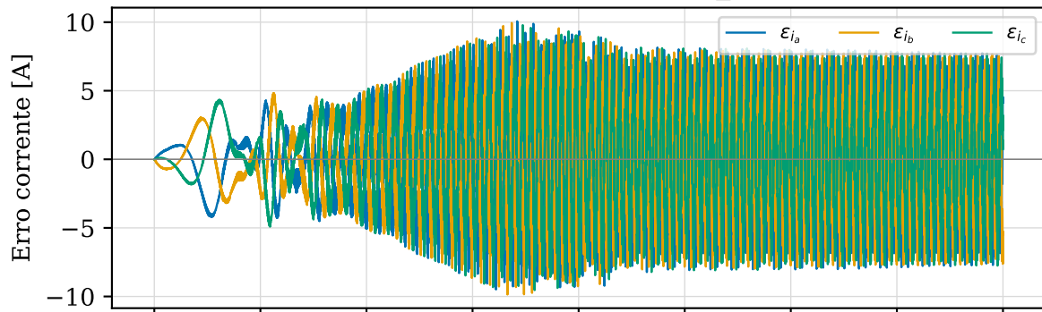
L3 — Full-stack — V/f 2 s: erro Top_HIL — C indep.
