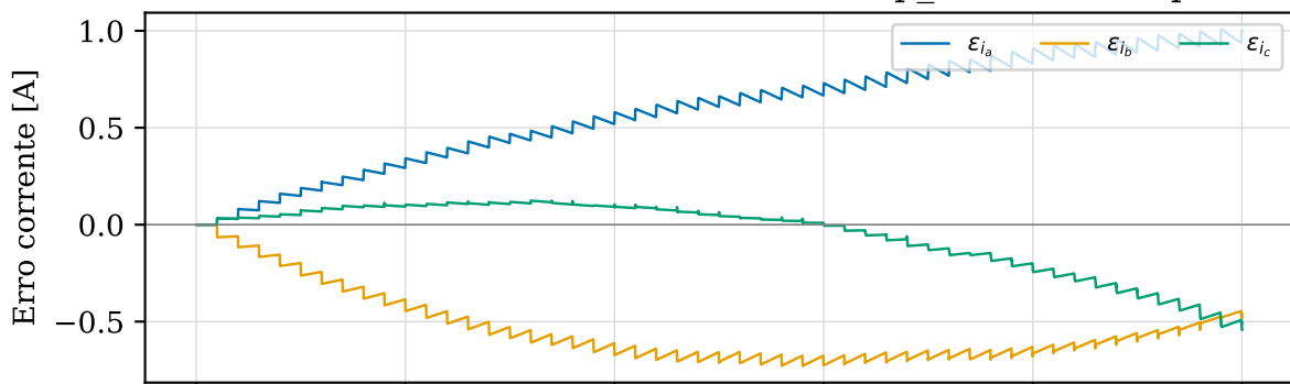
L3 — Full-stack — V/f 50 ms: erro Top_HIL — C indep.
