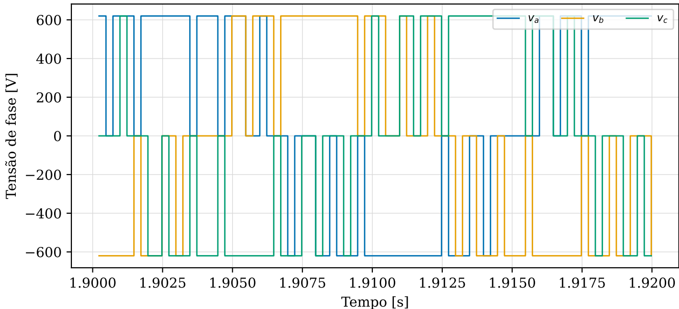
L3 — Full-stack — V/f 2 s: estímulo PWM (saída NPC), 1900–1920 ms
