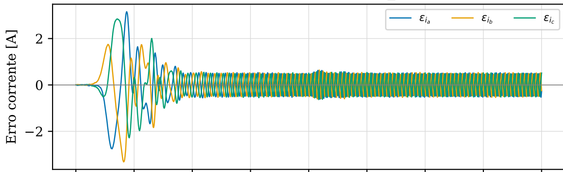
L3 — PWM replay — V/f 2 s: erro Top_HIL — C (replay)
