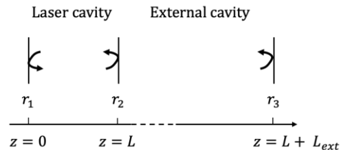
Fig. 1. Three-mirror cavity model for a laser diode with external feedback. r_1 and r_2 are the amplitude reflection coefficients at the back facet ( z=0 ) and front
