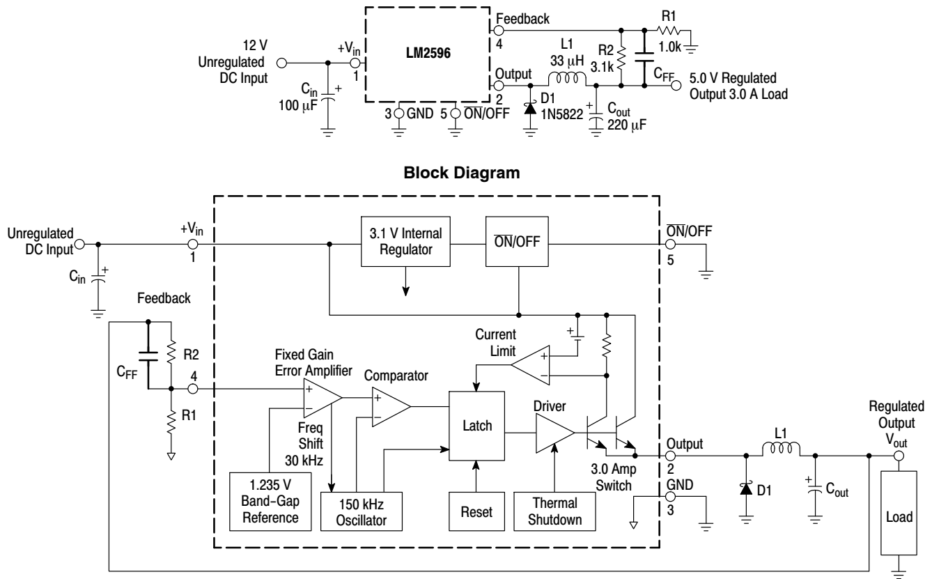
Figure 1. Typical Application and Internal Block Diagram
