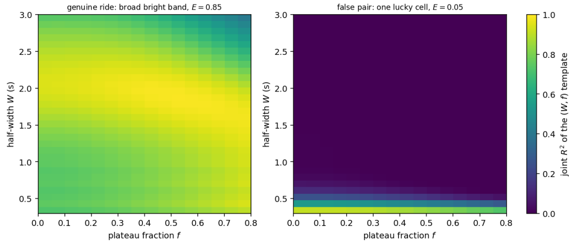
Fig. 14. The grid-energy gate e_{\min} . Each panel is the joint- R^2 heatmap over the (W, f) template grid for one candidate pair. A genuine ride (left) is a near-fit across a broad band of templates, so its grid energy E sits well above the 0.40 floor; a coincidental pairing (right) fits one narrow sliver and leaves the grid dark, so its energy falls far below the floor and Gate 4 rejects it.
