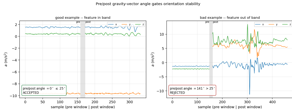
Fig. 19. Pre/post gravity-vector angle. Left: the gravity components hold level across the two rest windows, so one projection serves both ride ends. Right: the components jump between windows — the phone was reoriented mid-ride — and the tilt clears the 25^\circ gate.
