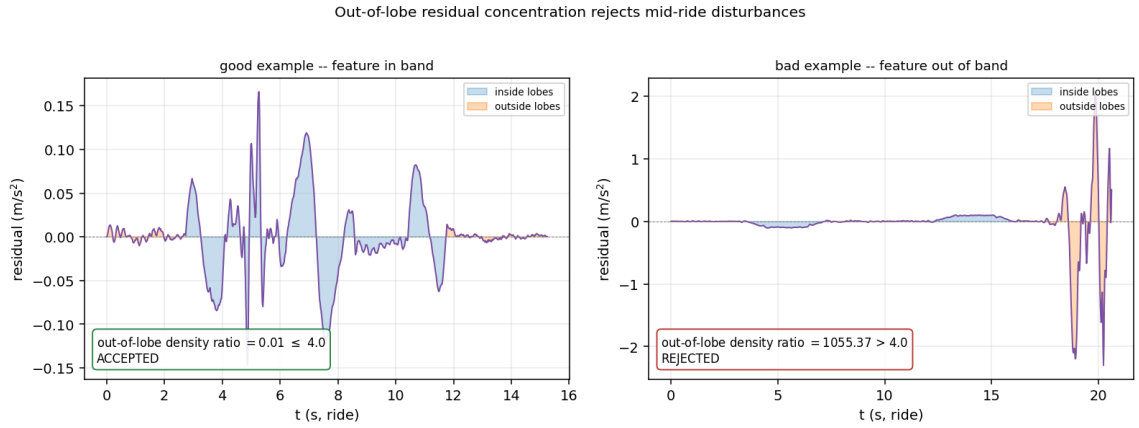
Fig. 25. Out-of-lobe residual concentration. Left: the residual energy stays within the two lobe windows. Right: residual energy concentrates outside the two lobe windows — a mid-ride disturbance the template never modelled.
