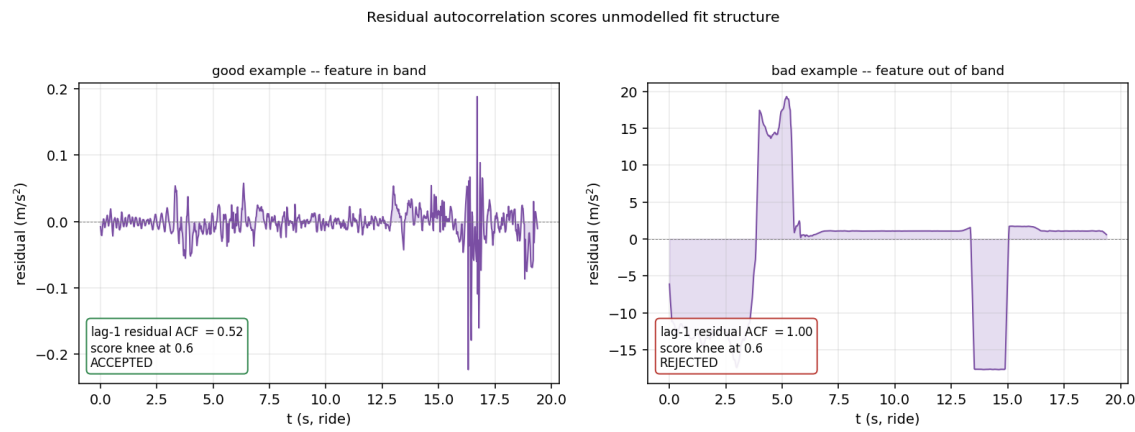
Fig. 23. Lag-1 residual autocorrelation. Left: the fit residual scatters tightly around zero. Right: the residual carries a slow, coherent excursion — structure the trapezoid template never modelled.
