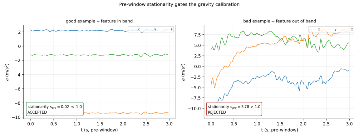
Fig. 18. Pre-window stationarity s_{pre} . Left: a still bracketing window — three flat axis traces — certifies the gravity calibration. Right: a window the filter cannot certify; the projection falls back to the unsigned magnitude and the ride is rejected.
