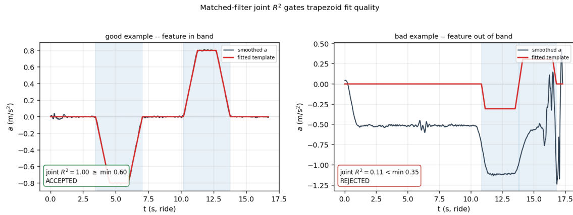
Fig. 22. Matched-filter joint R^2 . Left: the fitted trapezoid pair hugs the smoothed trace. Right: a trace with no clean pulse structure leaves the template far short of the graded R^2 floor.
