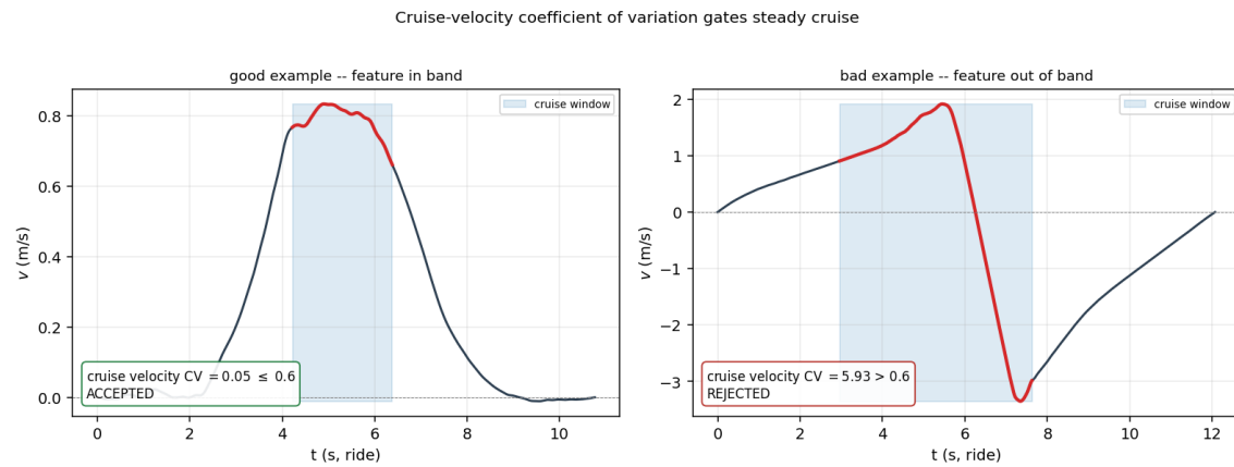
Fig. 26. Cruise-velocity coefficient of variation. Left: the ZUPT-integrated velocity holds a flat plateau between the lobes. Right: the plateau wobbles past the 0.6 gate — the cabin never settled into steady cruise.
