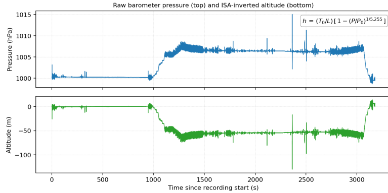
Fig. 10. Pressure ( top ) and the ISA-inverted altitude ( bottom ) on a Millennium-Hotel session. The pressure rise around t \approx 1000 s is the experimenter taking the elevator down from floor 12; the inverted altitude shows the matching \sim 50 m descent.
