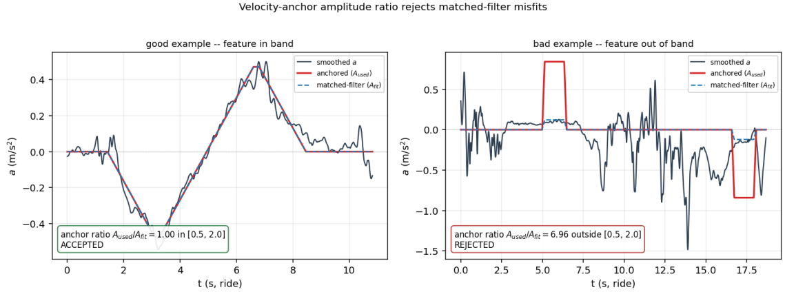
Fig. 24. Velocity-anchor amplitude ratio. Left: the velocity-anchored amplitude matches the matched-filter amplitude, so the two templates coincide. Right: the anchor rescales the amplitude far past the [0.5, 2.0] band — a matched-filter misfit.
