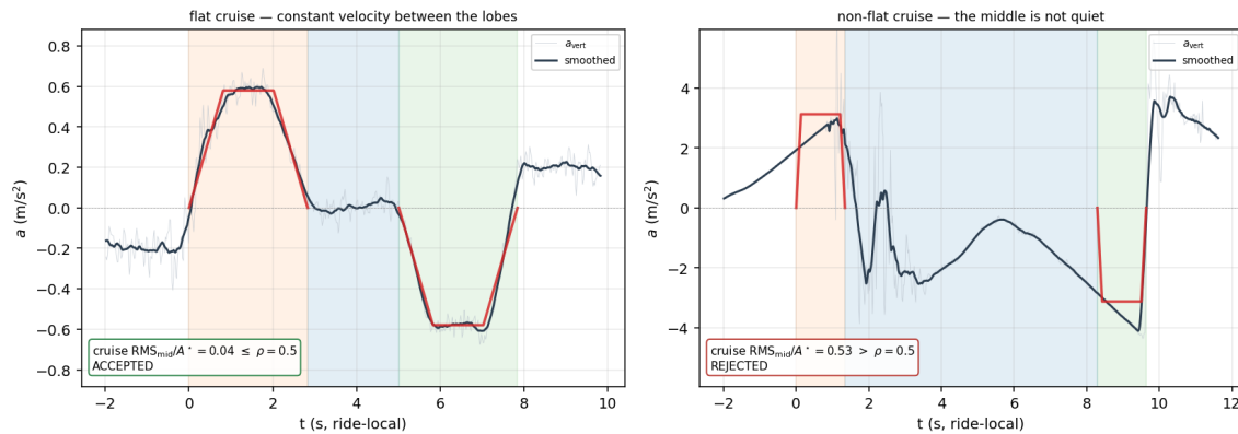
Fig. 15. The quiet-middle gate \rho . Left: a genuine ride — the smoothed acceleration returns to zero on the inter-lobe cruise (shaded), so \text{RMS}_{\text{mid}}/A^* stays well under \rho = 0.5 and the pair is accepted. Right: a pair whose inter-lobe stretch never goes quiet — \text{RMS}_{\text{mid}}/A^* exceeds 0.5 and Gate 5 rejects it.
