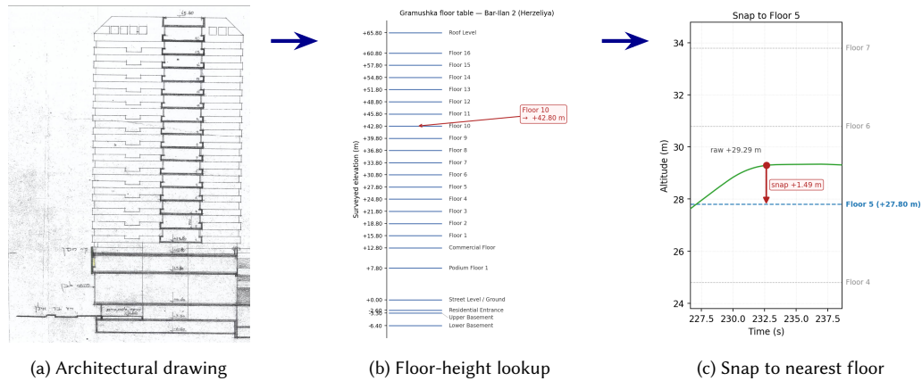
Fig. 12. From drawing to floor-height lookup to snapped ride endpoint. (a) The accordion-folded architectural section drawing for one campaign building (Bar-Ilan 2, Herzeliya). (b) The transcribed lookup, mapping each floor name to one surveyed elevation (annotated arrow: Floor 10 at +42.80 m). (c) A worked snap from a real Bar-Ilan 2 ride: the raw barometer altitude +29.29 m snaps +1.49 m down to Floor 5 at +27.80 m.
