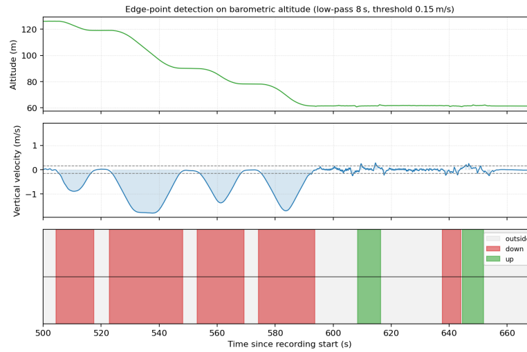
Fig. 11. Barometer interval detector on a 170 s window of Millennium-Hotel session exp2. Top: low-pass altitude. Middle: smoothed vertical velocity with the \pm 0.15 m/s threshold (dashed) and the “moving” regions shaded. Bottom: the surviving up/down intervals after merging, with outside between them.
