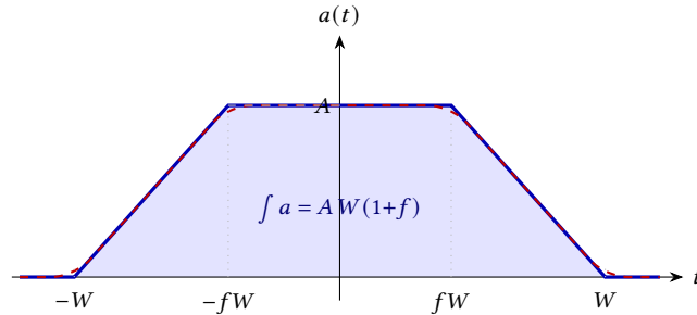
Fig. 17. One acceleration lobe of the S-curve. Under the bang-bang jerk command (3) the lobe is exactly the trapezoid \tau_{W,f} (solid), with (W, f) fixed by the machine parameters through (10)–(11). A controller that caps the jerk derivative rounds the four corners (dashed); the trapezoid is the area- and centroid-matched linearisation of that rounded lobe, so the shaded area A W (1 + f) — the cruise velocity — and the centroid are preserved, and with them the closed-form height (23).
