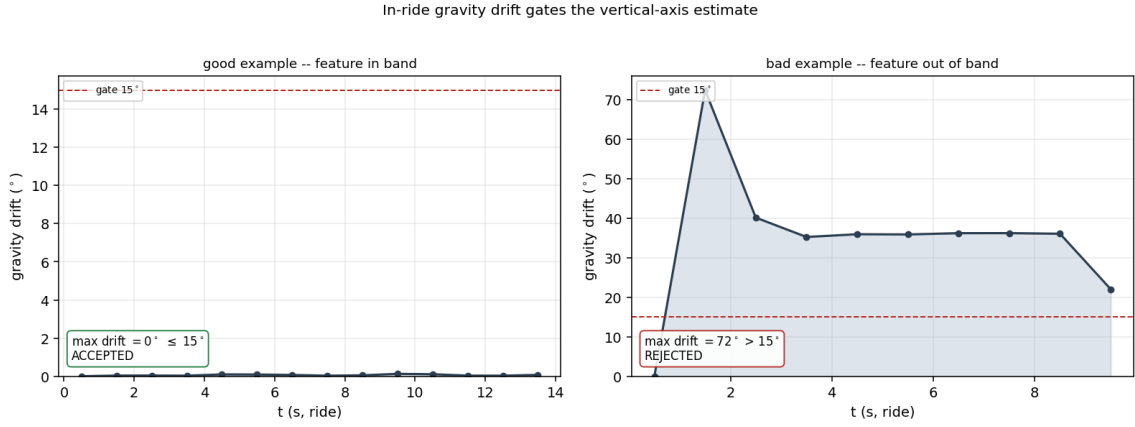
Fig. 20. In-ride gravity drift. Left: the gravity direction holds within a few degrees through the ride. Right: the direction sweeps past the 15° gate, so no single vertical axis describes the whole segment.
