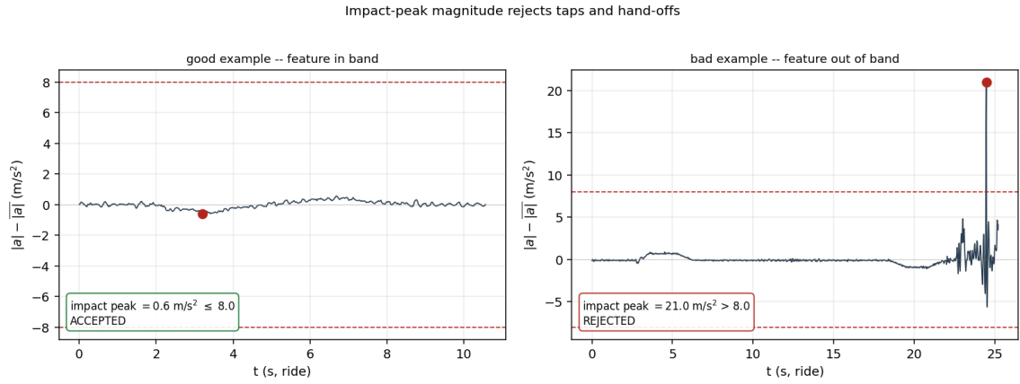
Fig. 21. Impact-peak magnitude. Left: the magnitude-detrended trace stays within the elevator's own acceleration band. Right: a hand-off spike clears the 8 m/s 2 gate; double integration would fold it into the height.
