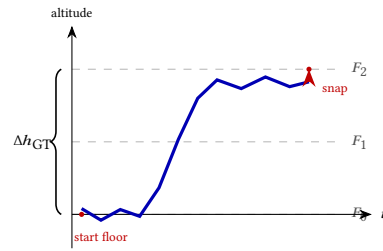
Fig. 6. Snapping the drifting barometer altitude (blue) to the nearest gramushka floor line (dashed) yields a drift-free ground-truth \Delta h .
