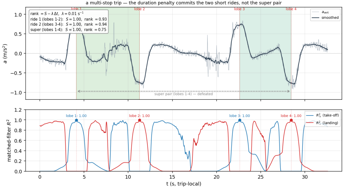
Fig. 16. The duration penalty \lambda on an up-going multi-stop trip. Top: the acceleration trace — four lobes, two back-to-back rides (shaded). Bottom: the matched-filter signed- R^2 score, peaking at all four lobes. The take-off of the first ride and the landing of the last form a super pair whose joint score S matches either short ride; only the rank S - \lambda \Delta t separates them, docking the long span hardest so the two short rides commit first.
