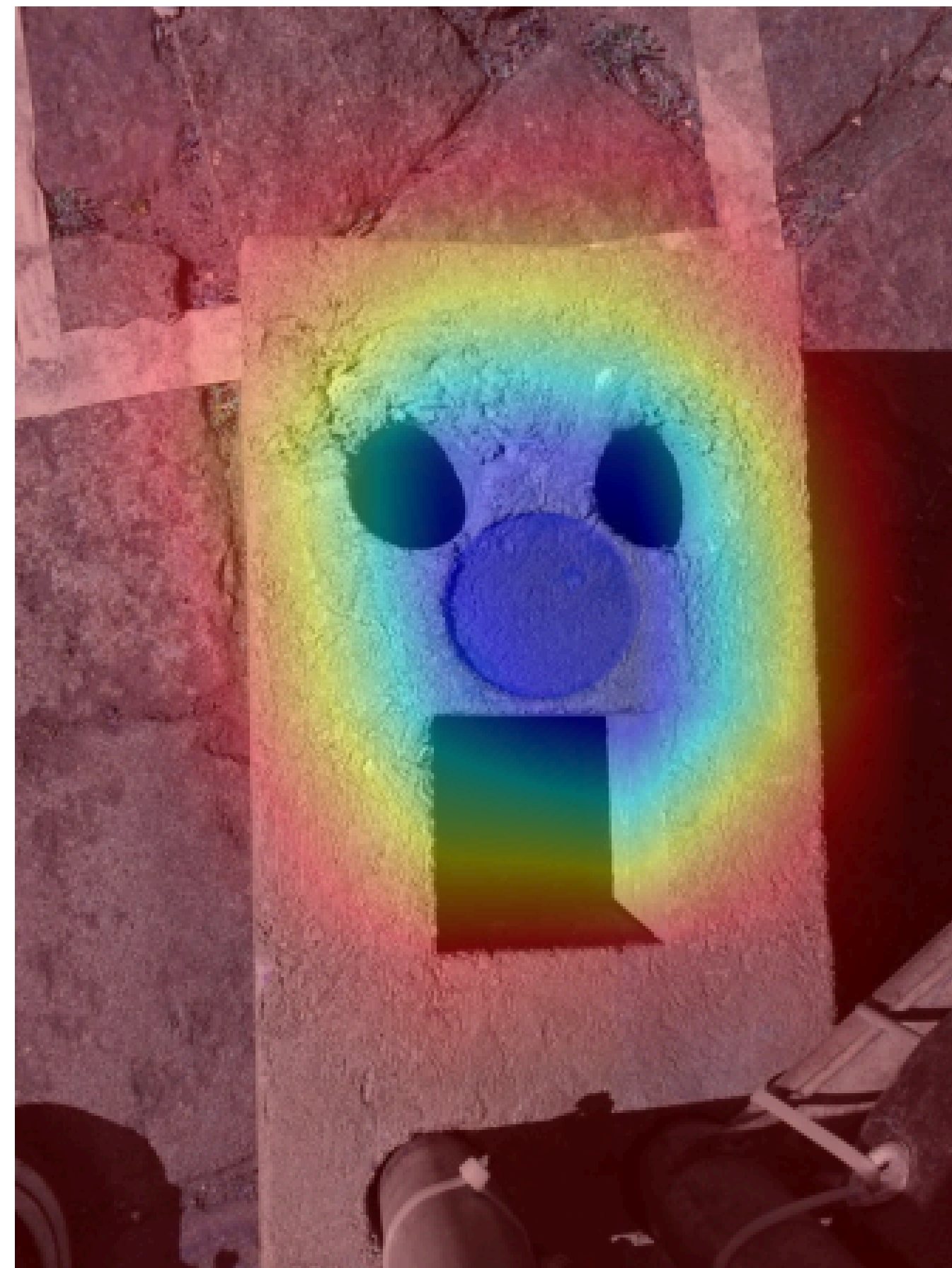
Grad-CAM
