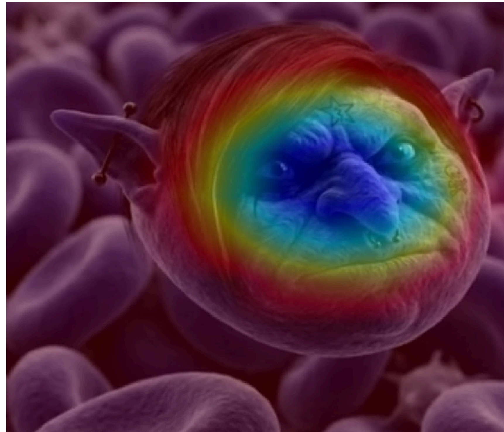
Grad-CAM
