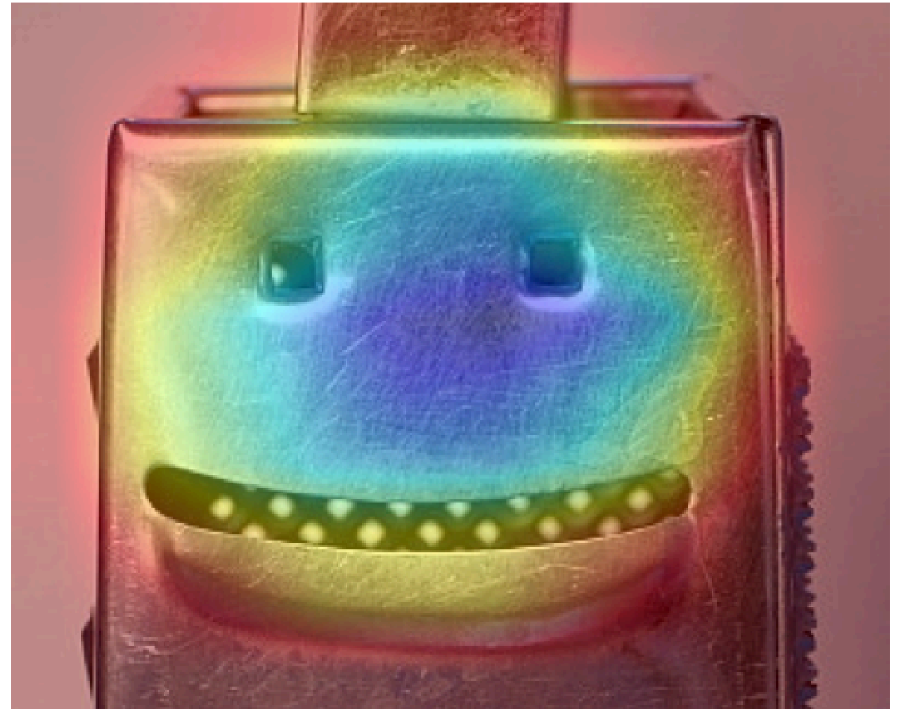
Grad-CAM
