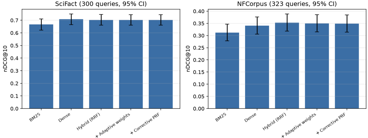
Figure 1: nDCG@10 across the ladder with 95% bootstrap confidence intervals.
