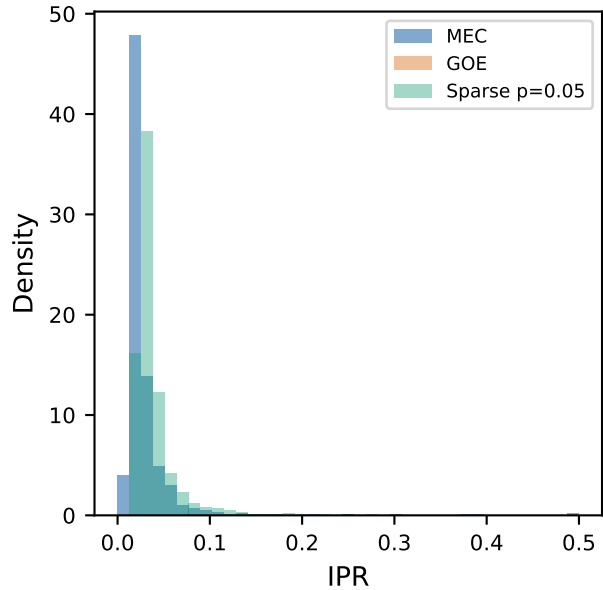
IPR distribution
