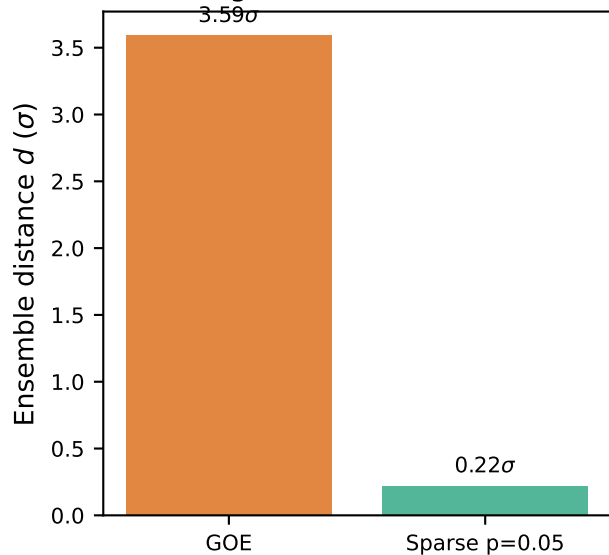
Eigenvector distance
