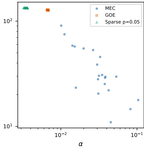
\alpha vs PR
