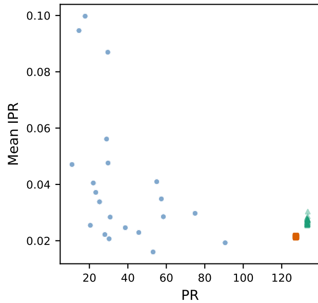
PR vs IPR
