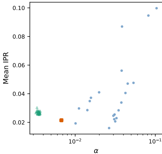
\alpha vs IPR
