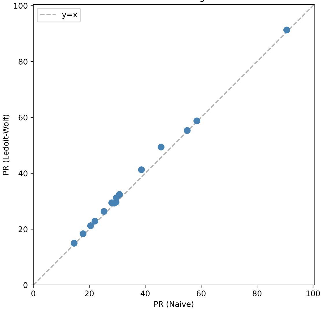
Naive vs Shrinkage PR
